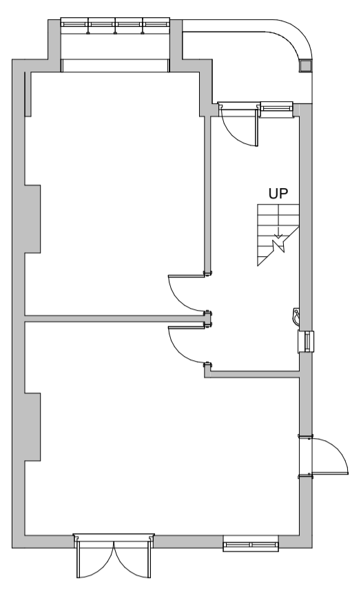
Existing Ground 1 : 100
