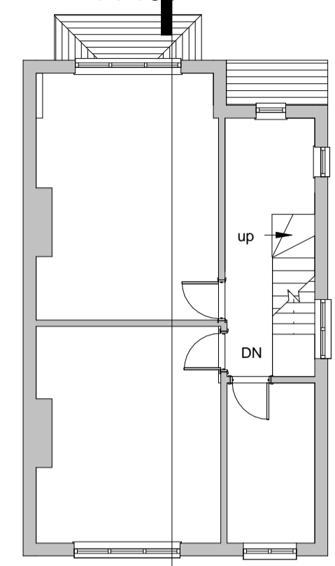
Proposed First 1 : 100
