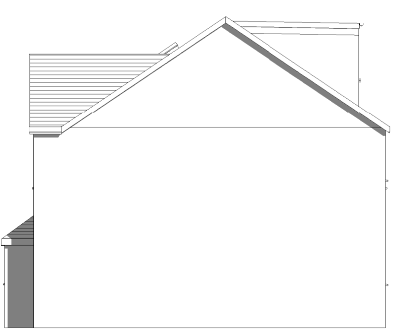
Proposed Side L 1 : 100
