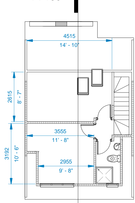
Proposed Second 1 : 100
